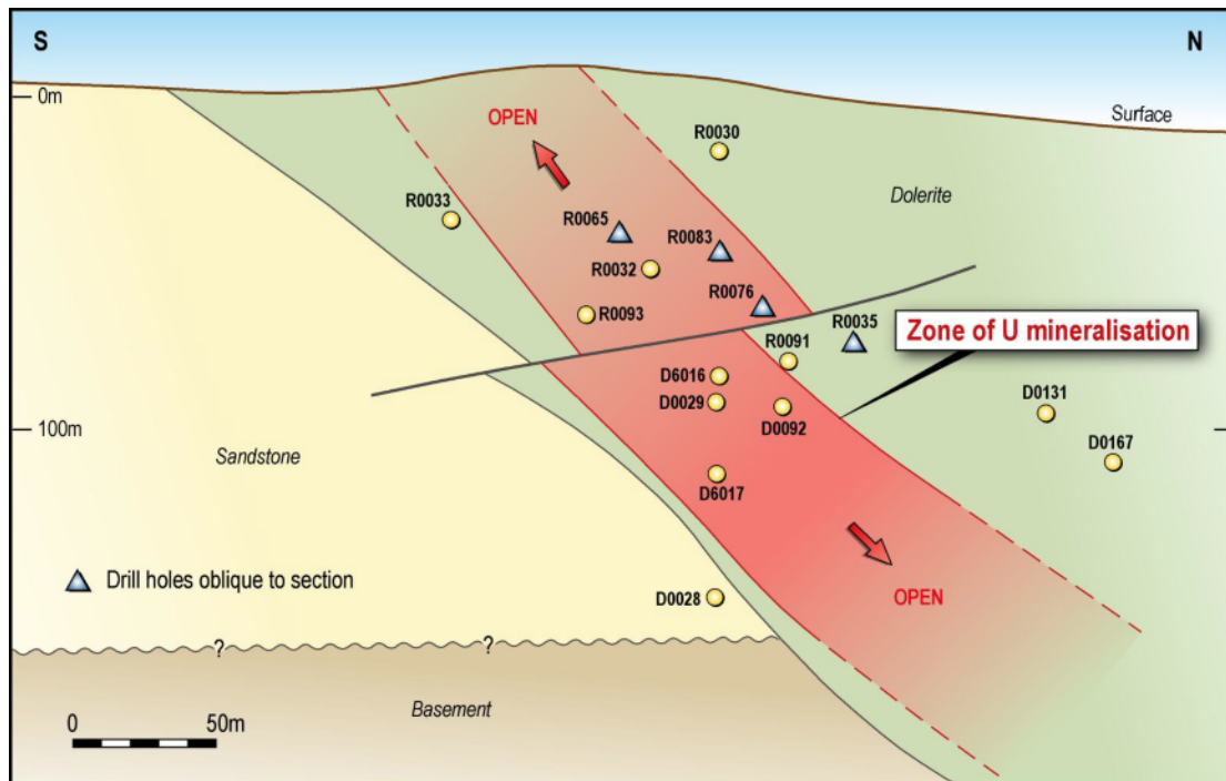
Figure 1: N147 Prospect Long Section with mineralisation open up and down plunge.
